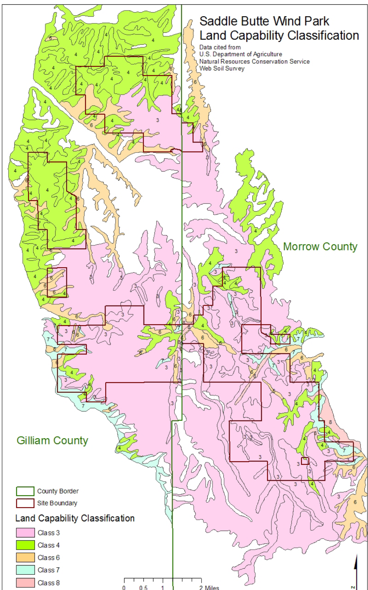
G-7 Land capability classification map
